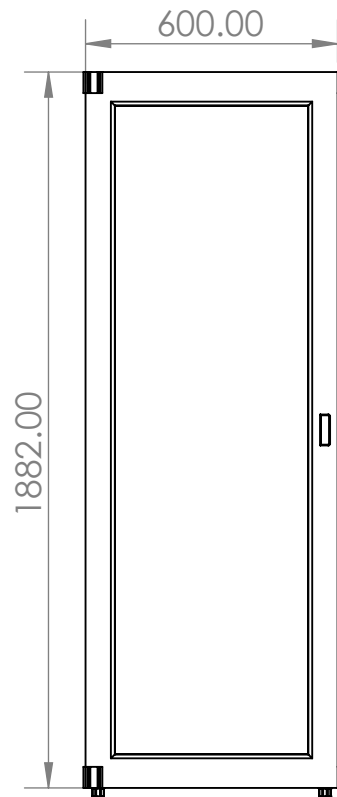
FRONT VIEW
